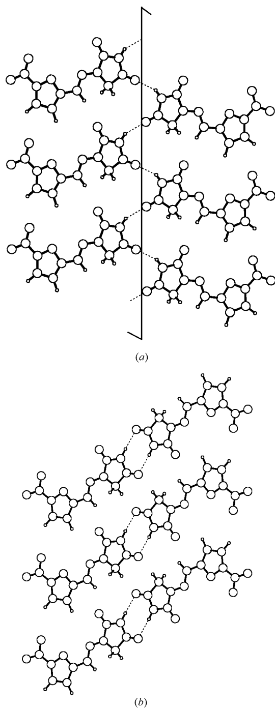
Figure 7 The triclinic (X \alpha ) and monoclinic (X \beta ) polymorphs of nitrofurantoin (Pienaar et al. , 1990a). A 180° rotation of the molecules on the right side of the helix (Fig. 6a) perpendicular to the twofold screw axis results in a rearrangement which forms R_2^2(8) dimers in the triclinic unit cell (Fig. 7b).
