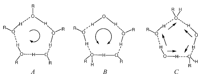
Figure 11 Homo-, anti- and heterodromic rings.
