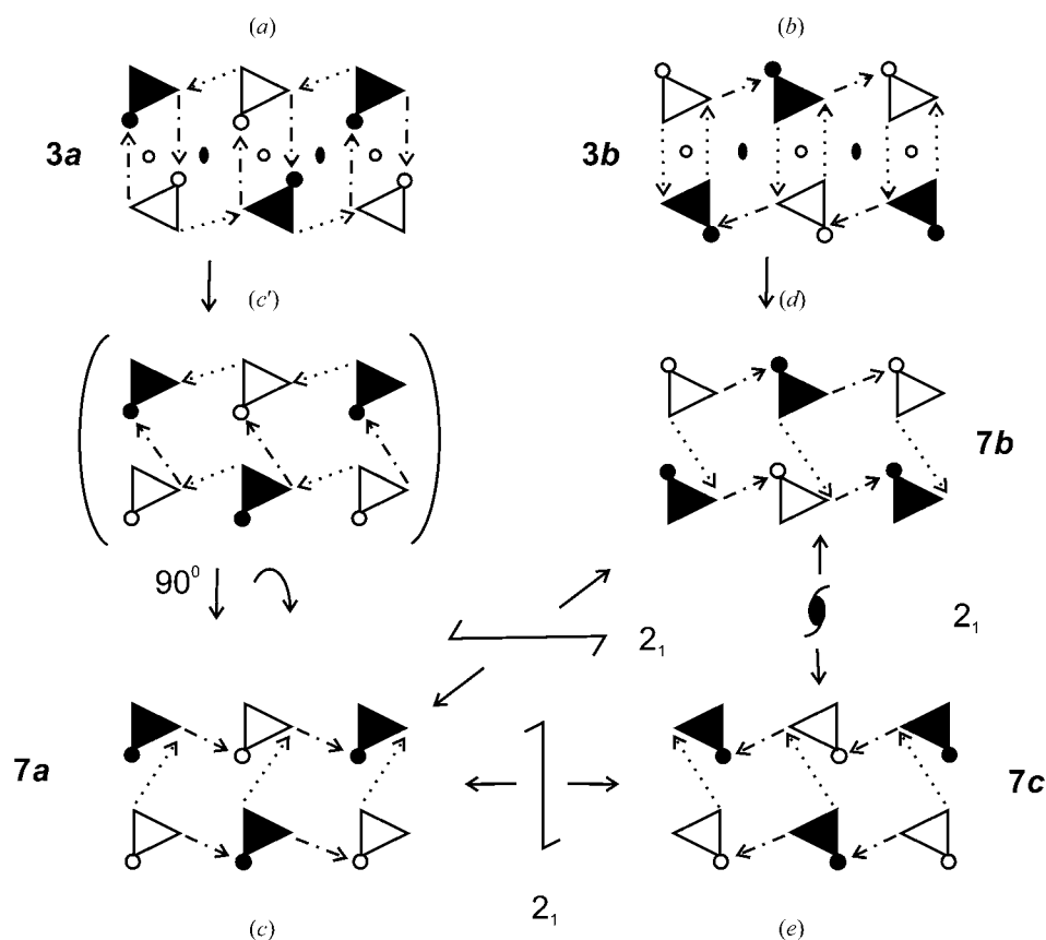
Figure 12 The parent sub-patterns (a) 3a and (b) 3b , and (c), (c'), (d) and (e) four different settings of pattern 7 formed by antidromic rings described by the graph-set notation R_4^4(18) .
