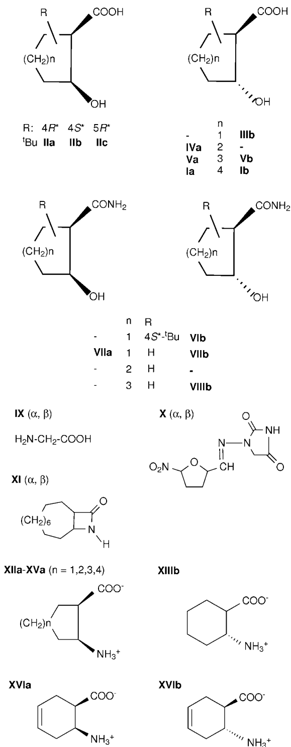
Figure 1 Chemical line drawings of the molecules labeled from (Ia) to (XVIb).
