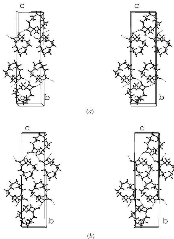
Figure 8 Stereoviews of the close packing of the polymorphs \alpha and \beta of (XI) in space group P2_1/c . In the unit cells (a) and (b), the positions of the cyclododecane rings are the same; only the positions of the C=O and N–H groups are interchanged. (Reproduced with kind permission from Fábíán et al. , 2004.)
