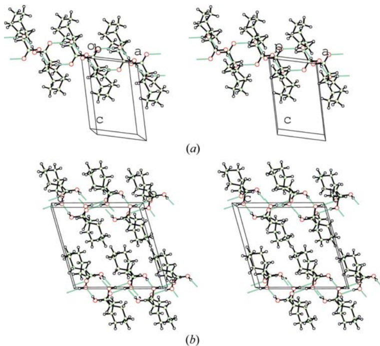
Figure 2 Stereoviews of the molecular packing of (Ib) ( P\bar{1} ) and (Ia) ( P2_1/c ). They are related by the type of rotation from 1 → 4b . Their common motif is the folded OC dimer located between planar OH dimers in (Ib) and between helices in (Ia). (Reproduced from Kálmán et al. , 2002b.)
